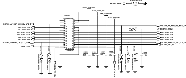
RCAM1_32M CAMERA(34PIN)
