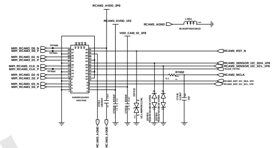
RCAM3_SUPER WIDE_8M CAMERA(30pin)
