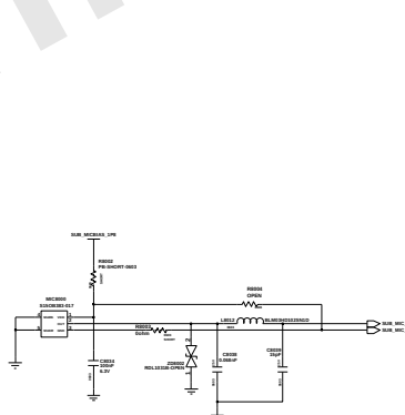
SUB MIC
