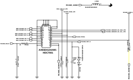
RCAM2_5M CAMERA(24PIN)
