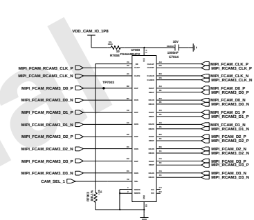
RCAM3_SUPER WIDE_8M CAMERA(30pin)
