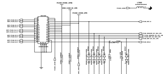
FRONT_32M CAMERA (30PIN)
